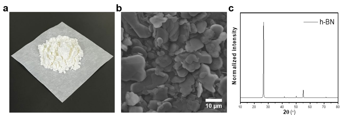
Fig S1. Elemental analysis of precursor h-BN: (a) optical image, (b) SEM image with low magnification, and (c) X-ray diffraction pattern.
