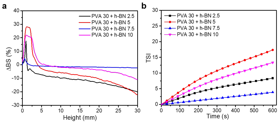
Fig S2. (a) Turbiscan analysis of slurries according to h-BN filler content (holding time: 10 minutes) (b) Turbiscan stability index (TSI) profiles of h-BN slurries over time filler content.
