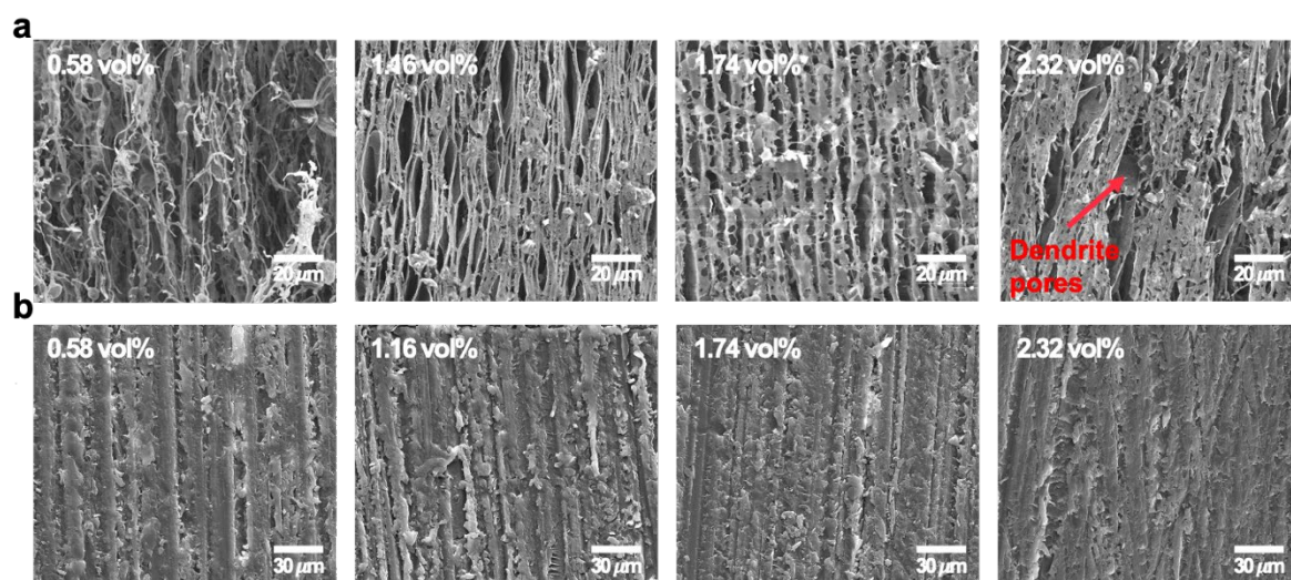
Fig S3. SEM images of (a) 3D h-BN structures based on filler content, (b) h-BN/epoxy composite based on filler content before compressive strength.
